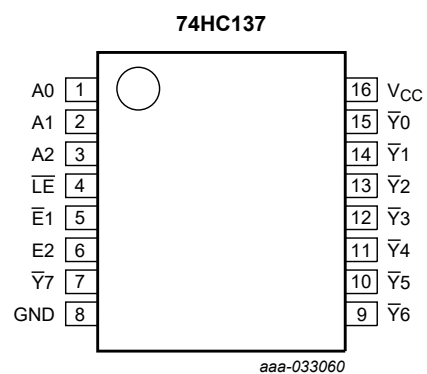
Fig. 6. Pin configuration SOT338-1 (SSOP16) and SOT403-1 (TSSOP16)
